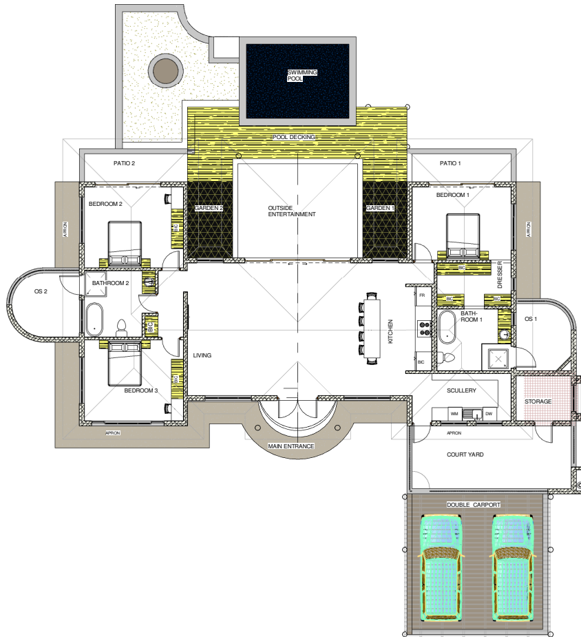
1 DIM PLAN GROUNDSTOREY NTS
