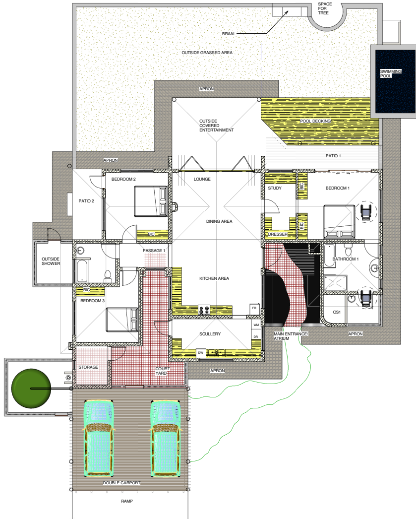
1 DIM PLAN GROUNDSTOREY
