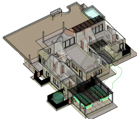
5 BIRD EYE VIEW - NO ROOF
